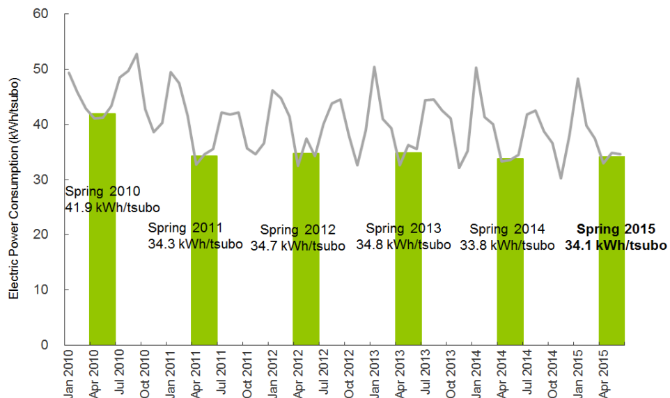
Figure 2: Average Electric Power Consumption by Office Tenants in Spring (April-June) (TEPCO area)
